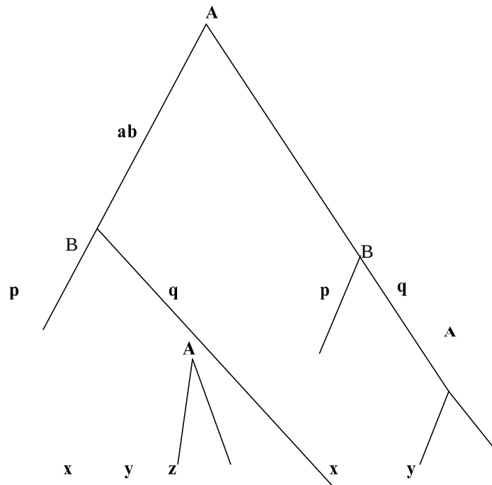
Figure 1: Structure of a simple game tree (extensive form model)
